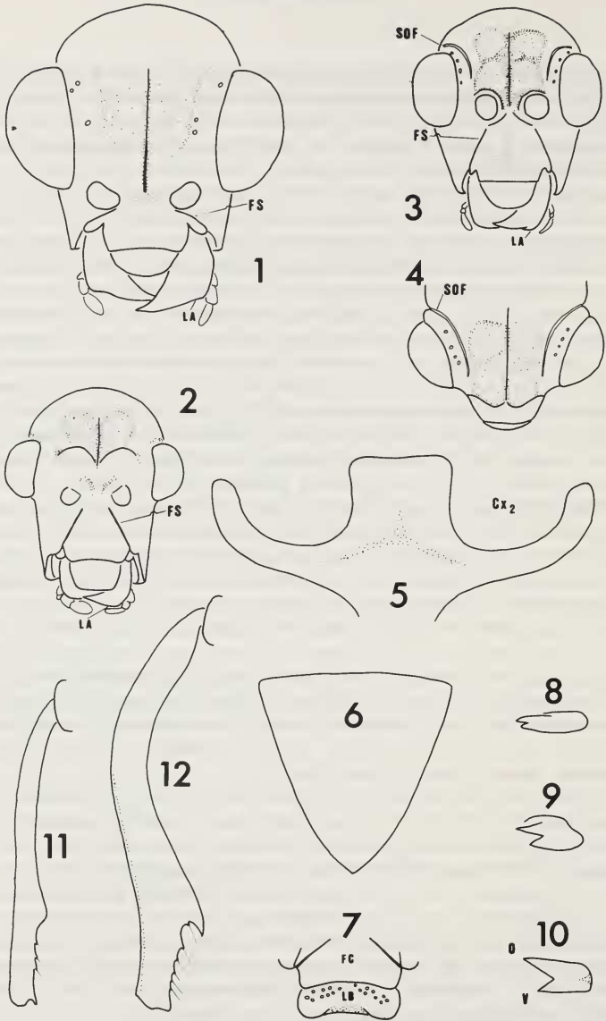
FIGURES 1-12: 1. Frontal aspect of head of Donacia hypoleuca Lacordaire. 2. Frontal aspect of head of Macrolepta pubipennis (Reuter). 3. Frontal aspect of head of Donaciasta luridiventris (Lacordaire). 4. Dorsal aspect of head of Donaciasta luridiventris . 5. Mesosternum of Donacia cincticornis Newman. 6. Pygium of female of Donacia cincticornis 7. Frontal aspect of frontoclypeus and labrum of Sominella kraatzi (Weise). 8. Apical aspect of left mandible of Plateumaris rufa (Say). 9. Apical aspect of left mandible of Poecilocera harrisii (LeConte). 10. Apical aspect of left mandible of Donacia cincticornis . 11. Lateral aspect of metatibia of female of Sominella macrocnemia (Fisch. v. Wald.). 12. Lateral aspect of left metatibia of male of Sominella macrocnemia . Cx 2 = mesocoxa; D = dorsal apical tooth of mandible; FC = frontoclypeus; FS = frontoclypeal suture; LA = lateral angulation of mandible; LB = labrum; SOF = supraocular furrow; V = ventral apical tooth of mandible. Scale bar = 1.0 mm for Figs. 1-10, 0.5 mm for Figs. 11 and 12.
